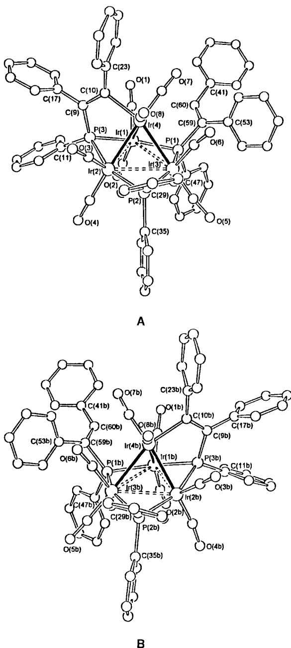
Fig. 1 Molecular structure of [\text{Ir}_4(\text{CO})_8(\mu_3\text{-}\eta^2\text{-PhPCPh=CPh})\text{-(}\mu\text{-PhPCPh=CHPh)(}\mu\text{-PPh}_2\text{)]} 2 (isomers A and B).
